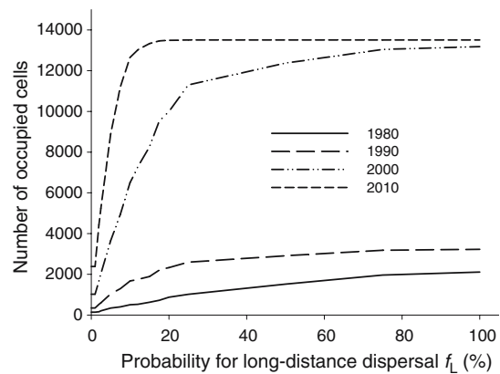
Fig. 5 Number of occupied cells for 1980, 1990, 2000, and 2010 in relation to the implemented probability for long-distance dispersal ( f_L ). Lower probabilities have over-proportionally higher effect on cell occupation than high probabilities
